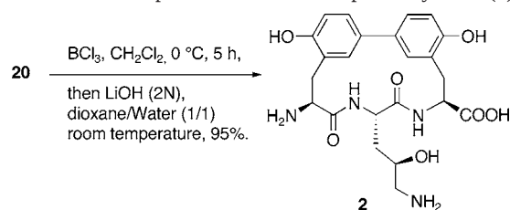
Scheme 4. Deprotection of 20 to Biphenomycin B ( 2 )
